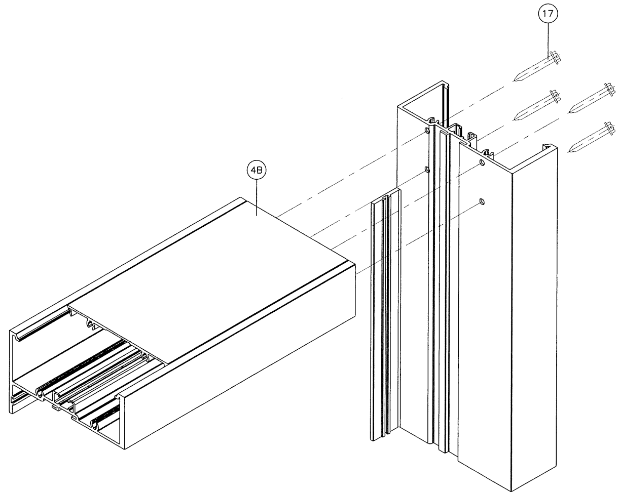
TOP/BOTTOM CORNERS
