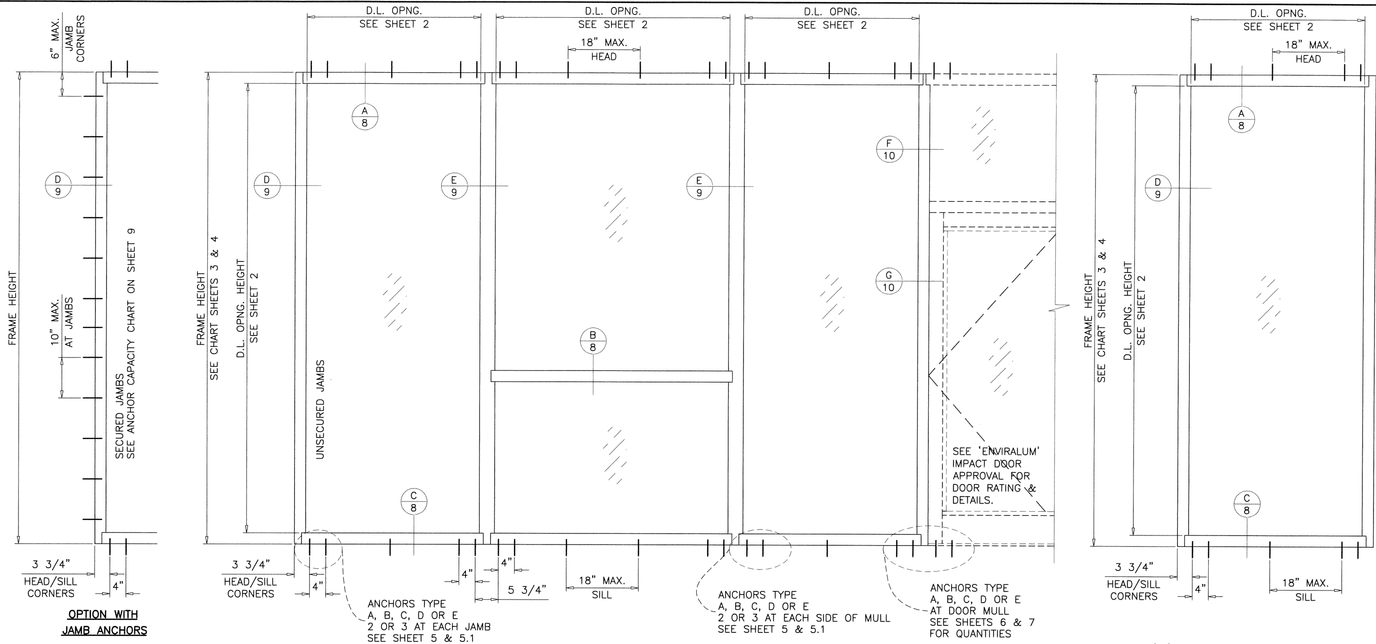
TYPICAL ELEVATIONS
